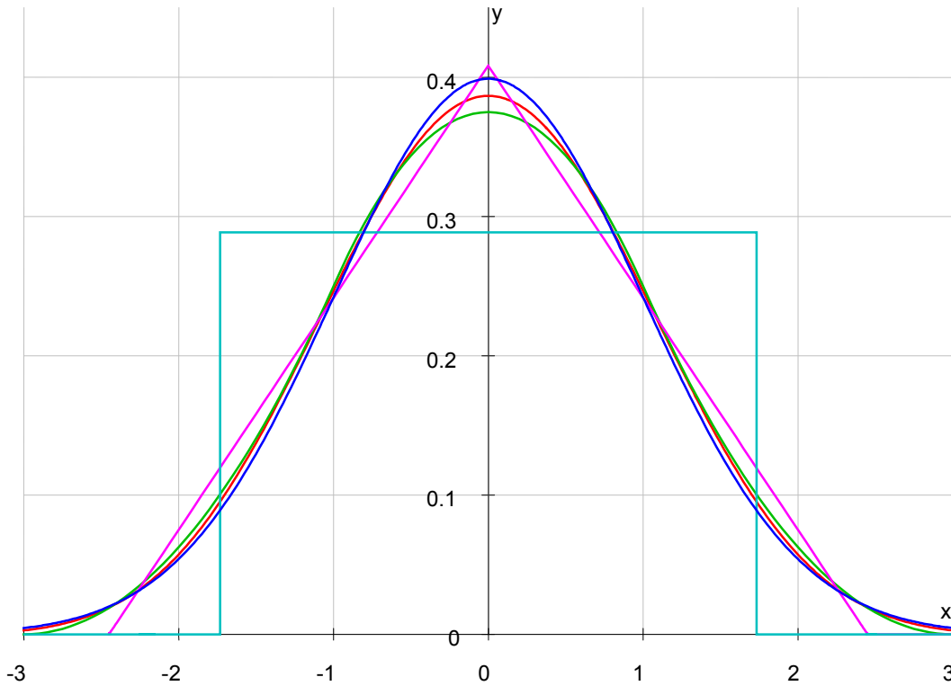
Picture 14: n^{\text{th}} degree approximation a. Gaussian blur b. 1 st degree, box blur c. 2 nd degree, linear blur d. 3 rd degree, square blur e. 5 th degree, quadruple blur
